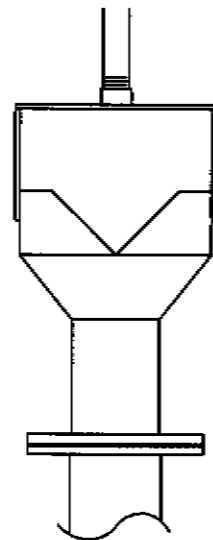
Funnel w/vee notches 180° apart
